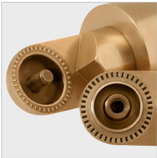
INTERLOCK MECHANISM Our directional lights feature a precision-engineered rotation mechanism with cast notches for superior durability and wear resistance. Designed for longevity, it also includes a threaded stud that can be easily replaced in the field.
