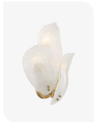
3 LIGHT WALL SCONCE ▲ N2213-732 - White Glass N2213-A-732 - Amber Glass 13" W x 18.25" H x 6" Ext. 3 - 60W E12 Candelabra Base Dimmable
