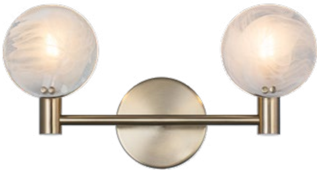
W33802CG Dimension. 15 1/2"W x 8"H x 4 3/8"E Lamping. 2x10W Candelabra Base-E12 120V Canopy. Ø4 3/4" x 7/8"E H/CTR. 5 5/8"
