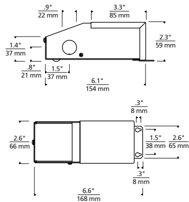
60W AND 100W MLV ENCLOSURE
