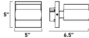
E30161-10BK Wall Mount
