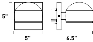
E30164-BK Wall Mount
