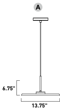
E34001-AB, -ACP, -BK Pendant
