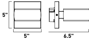
E30160-BK Interior/Exterior Wall Sconce
