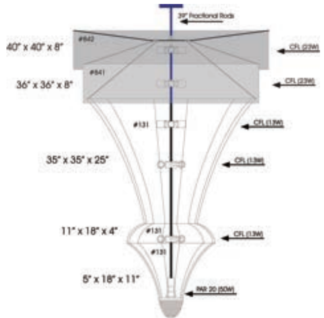
CAD Rendering
