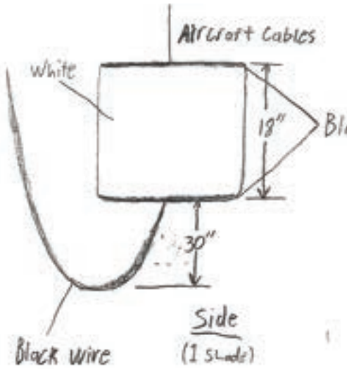
Designer's Sketch
