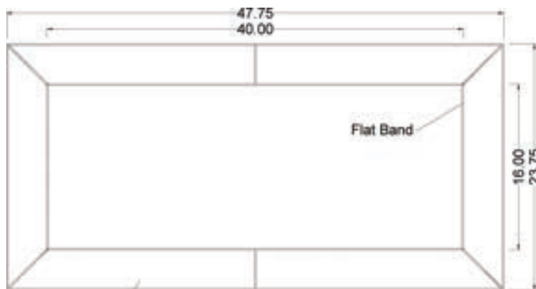
Fixed "Diffuser"
