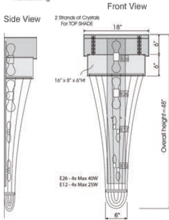
CAD Rendering
