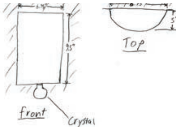
Designer's Sketch
