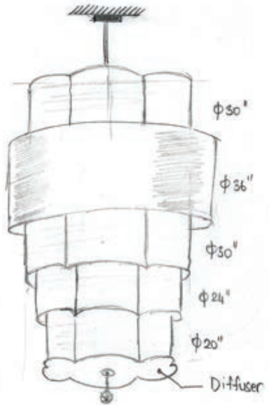
CAD Rendering
