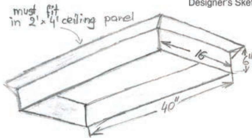
Designer's Sketch
